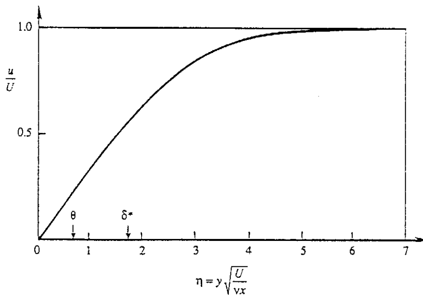
Figure 10.7 The Blasius similarity solution of velocity distribution in a laminar boundary layer on a flat plate. The momentum thickness \theta and displacement \delta^* are indicated by arrows on the horizontal axis.
